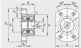
ZKLFA...-2RS、ZKLFA...-2Z
