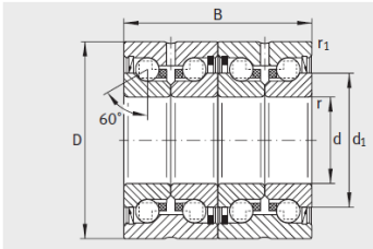
ZKLN..-2RS-2AP
