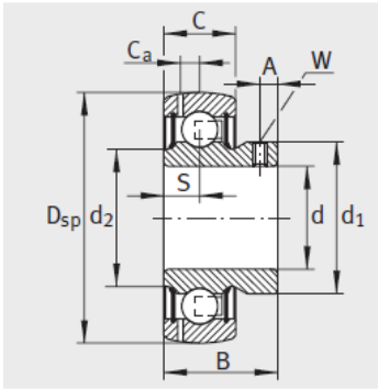
GAY12-NPP-B、AY12-NPP-B
